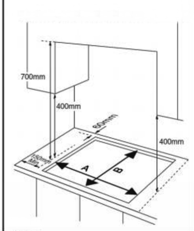
CLEARANCES REQUIRED WHEN FITTING THE HOB WITHOUT A COOKER HOOD ABOVE
